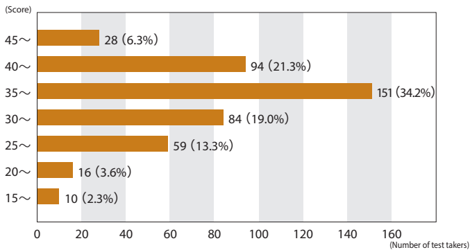
Writing score (All test takers) (442)
