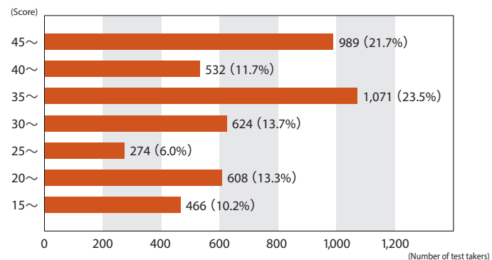
Writing score (All test takers) (4,564)
