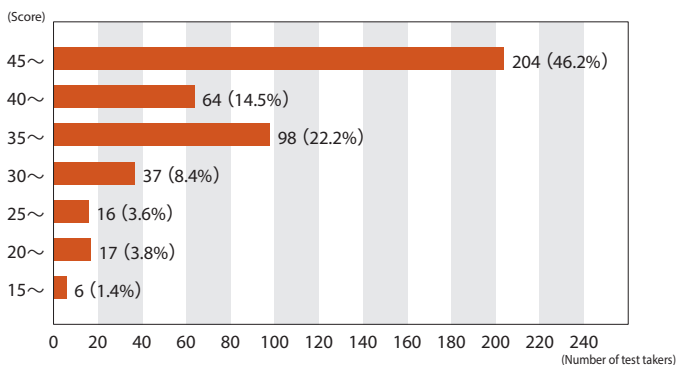
Writing score (All test takers) (442)
