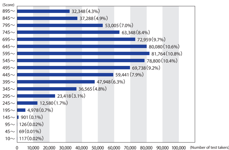
I-3. Total score distribution (SP)
