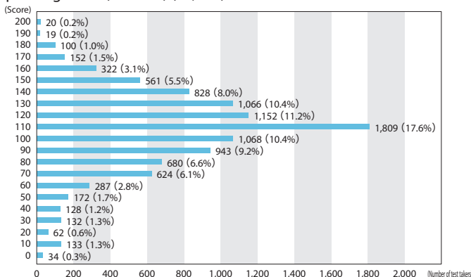
Speaking score (Schools) (10,292)
