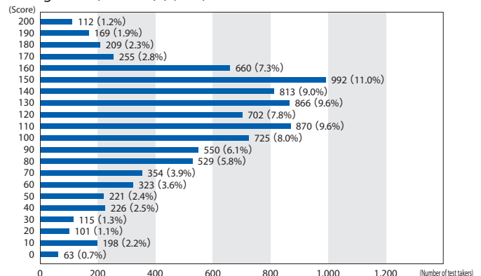
Writing score (Schools) (9,053)
