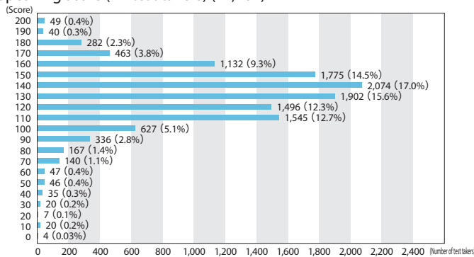
I-3. Score distribution (SP)
